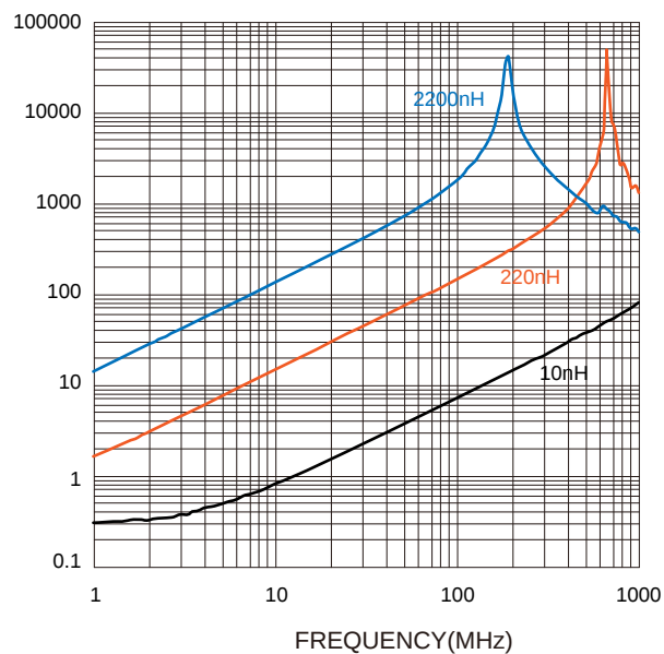
Impedance VS. Frequency Characteristics:
