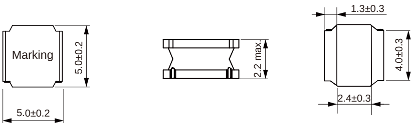
Dimensions: [mm]
