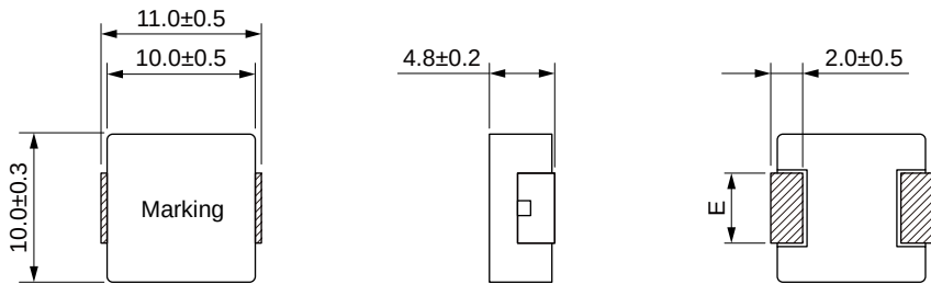
Dimensions: [mm]
